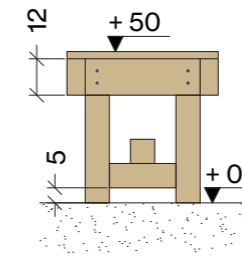
View bench A-A'
