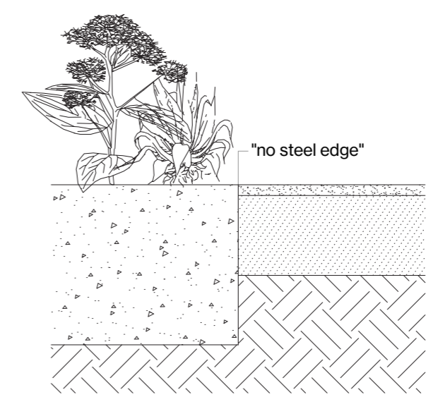
Transition between planting area (left) and path (right) - M 1:10
