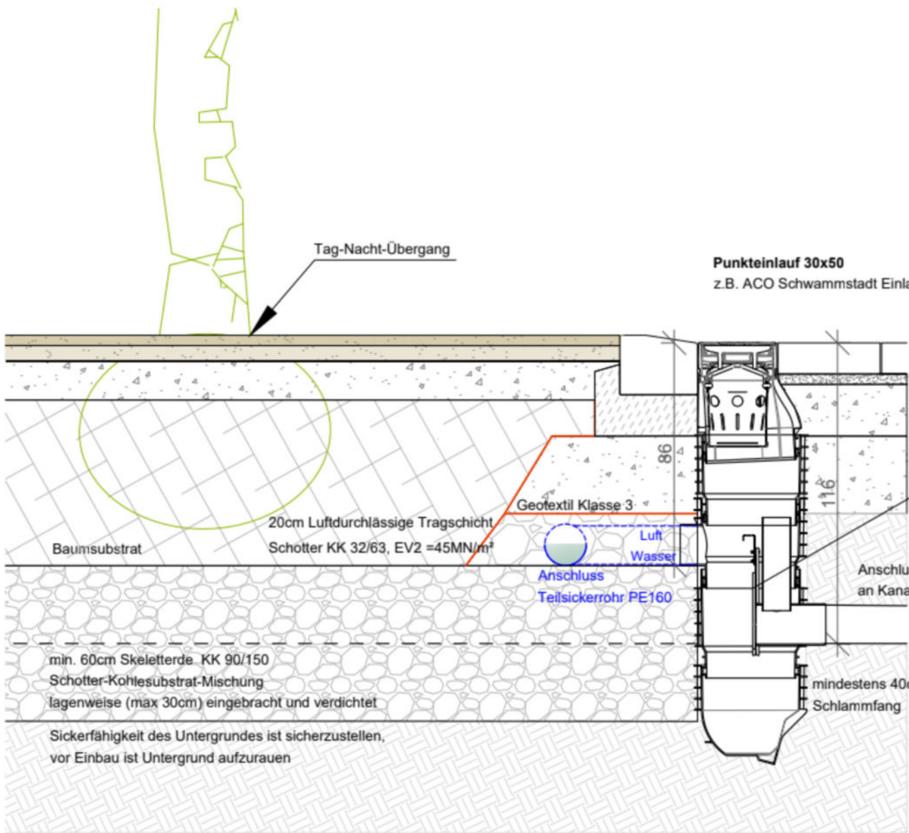
DETAIL 1:20
